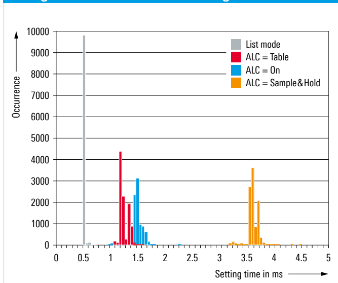
Histogram of measured level setting times in I/Q mode
