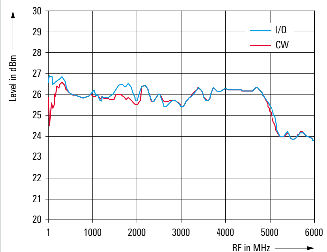
Measured maximum output power versus frequency
